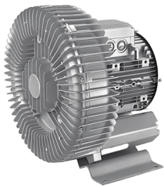
Légfúvó 310T 0,7kW/400V, 100m 3 /h 150mbar
